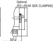
MODEL J-260-ND-SL SINGLE SIDE SLOTTED FLEXMOUNT Ø27mm TO 46mm = SF4
