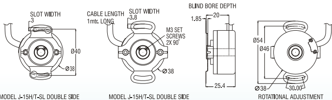
MODEL J-15H/T-SL DOUBLE SIDE SLOTTED FLEX MOUNT \varnothing 40mm = SF7
